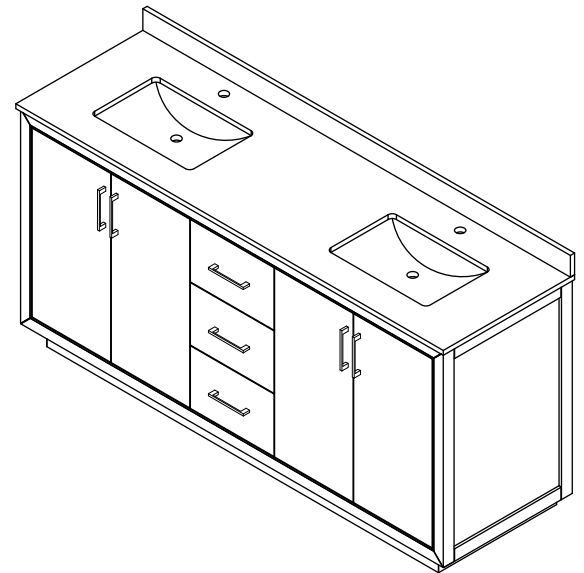
Technical drawing of a cabinet with the following dimensions: Overall width: 71" Overall height: 21-3/4" Left panel width: 27-1/4" Door width: 13-1/2" Right panel width: 27-1/4" Left panel height: 16-1/2" Door height: 15-1/2" Door width (inner): 12-3/4"
