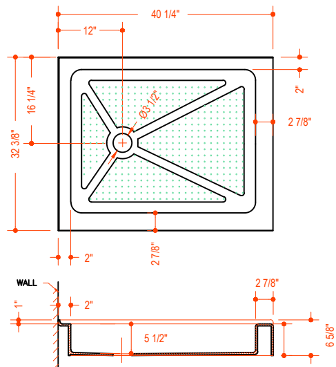
MODEL VG06019XXX3240*
