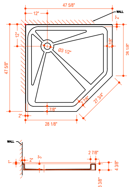
MODEL VG06068XXX4747
