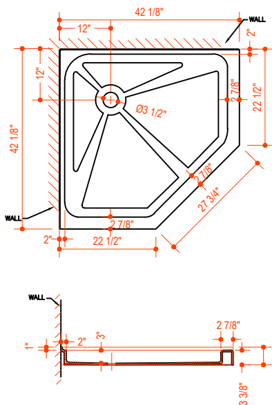
MODEL VG06068XXX4242
