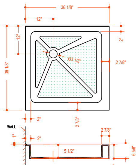
MODEL VG06019XXX3636
