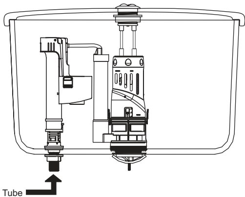
Connect Water supply Tube
