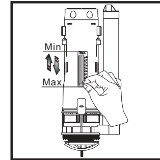
Adjustment of whole flush level: when the white card is on the highest position, the whole flush water is at the least.
