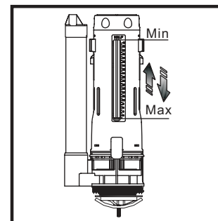
Adjustment of partial flush level: The partial flush float is higher, the partial flush water is less.
