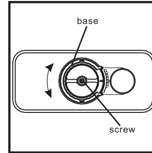
Install the flush valve base into the outlet to make the "U" clasp on the tank properly. Rotate the base to choose proper angle and lock the screw.
