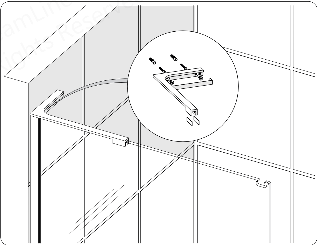
Fig 14 Left-hand L-Bar™ Support Bracket shown*
