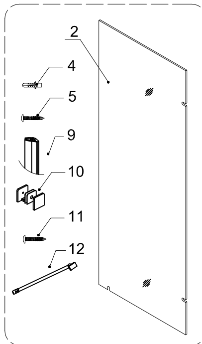
Stationary Glass Panel with Top Brace
