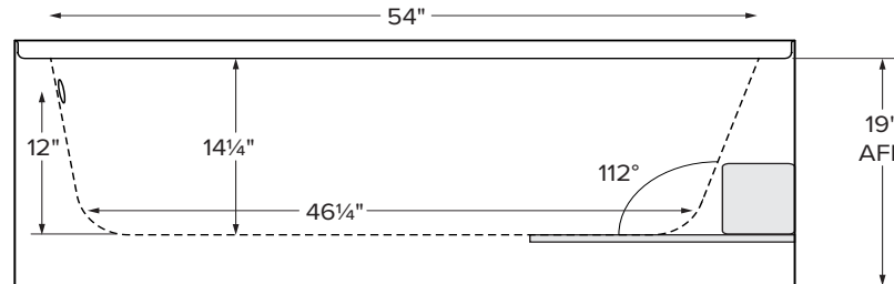
This tub model features a 19" skirt height that allows for above floor rough-in.
