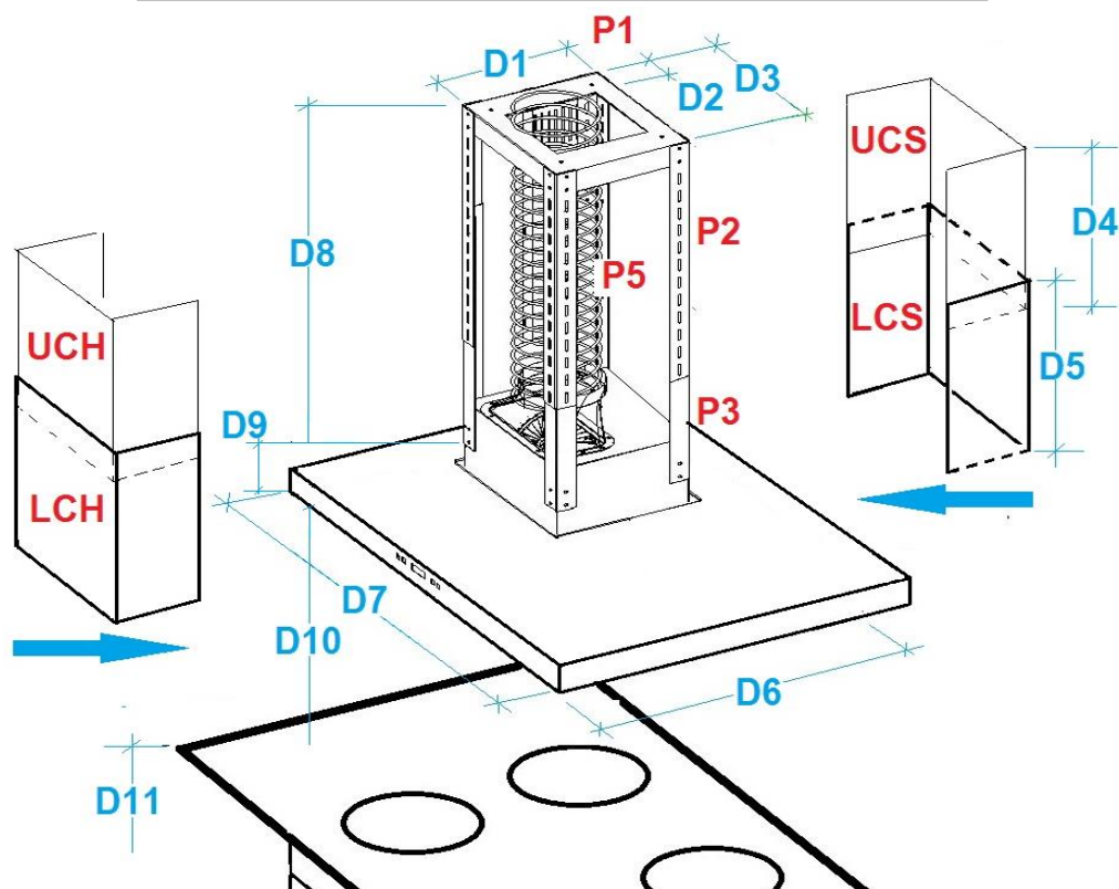
DIMENSION TABLE
