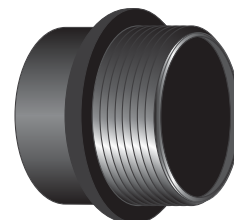
Male Adapter Spg x MIPT - ABS DWV for Aquatica® bath wastes with Sch40 hub outlet. Thread: 1 1/2 NPSM (1 1/2 IPS)
