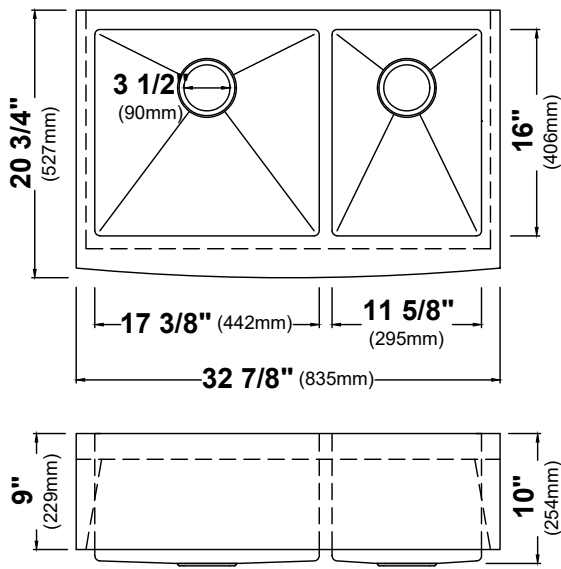
Model #: KHF203-33 Sink Dimensions: 32 7/8" x 20 3/4" x 10" Min Cabinet Size: 33"
