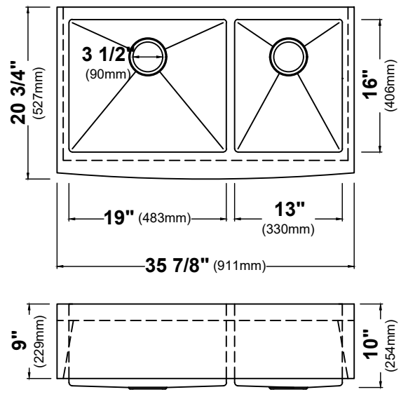
Model #: KHF203-36 Sink Dimensions: 35 7/8" x 20 3/4" x 10" Min Cabinet Size: 36"
