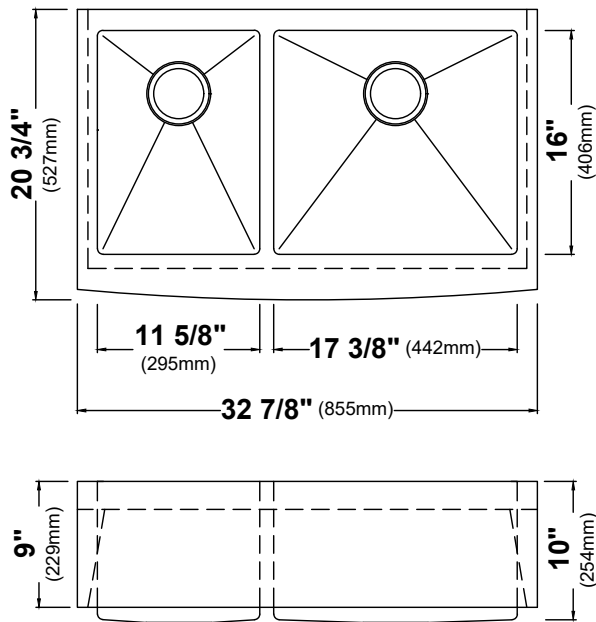
Model #: KHF204-33 Sink Dimensions: 32 7/8" x 20 3/4" x 10" Min Cabinet Size: 33"
