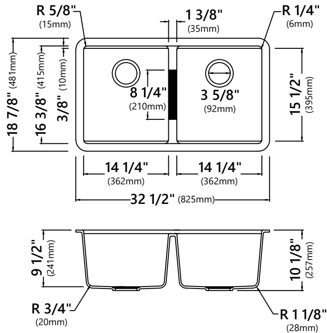
Model #: KGU-434B Sink Dimensions: 33" x 22" x 9 1/2" Min Cabinet Size: 36"
