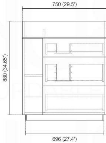
FRONT ELEVATION
