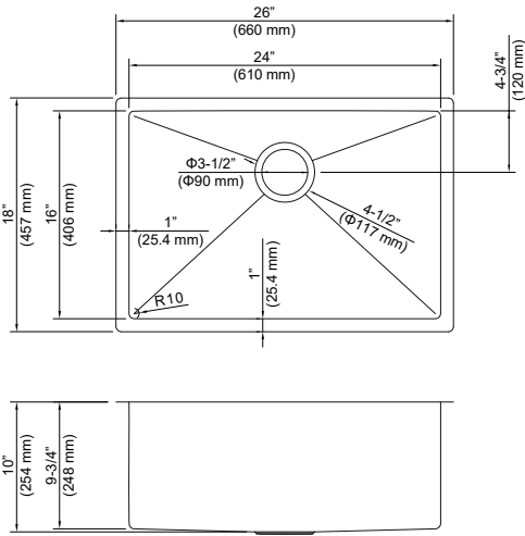
K1-S26 26"X18"X10" Min Cabinet Size: 30"
