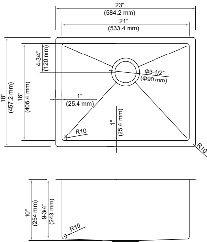
K1-S23 23"X18"X10" Min Cabinet Size: 27"
