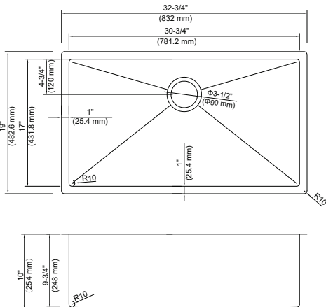
K1-S33 32-3/4"X19"X10" Min Cabinet Size: 36"
