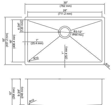
K1-S30 30"X18"X10" Min Cabinet Size: 33"
