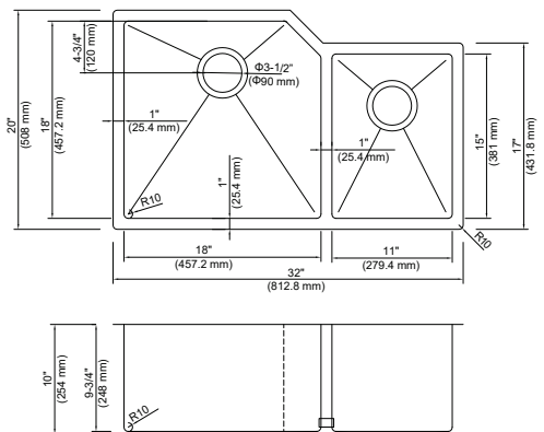
K1-D32 32"X20"X10" Min Cabinet Size: 36"
