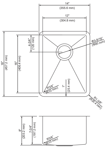
K1-S14 14"X18"X8" Min Cabinet Size: 18"
