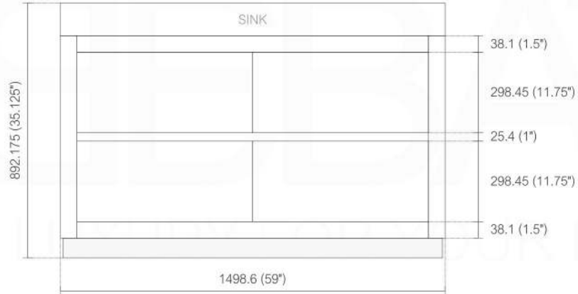
BACK ELEVATION
