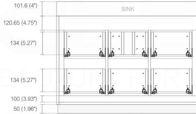
BACK ELEVATION
