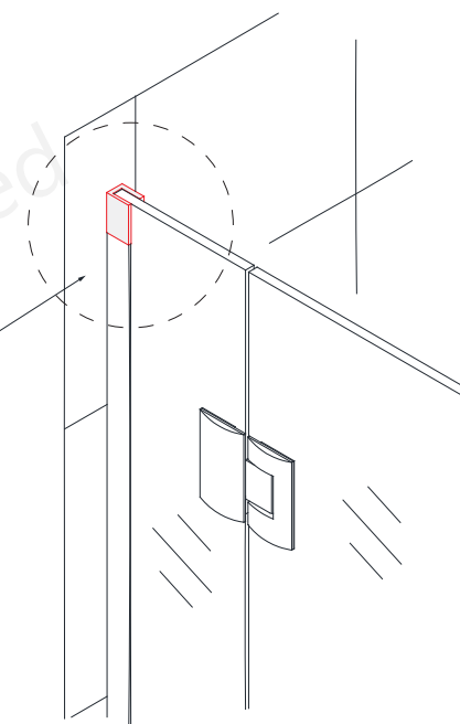
6" Hinge Panel with Hinge Panel Glass Bracket (#36)
