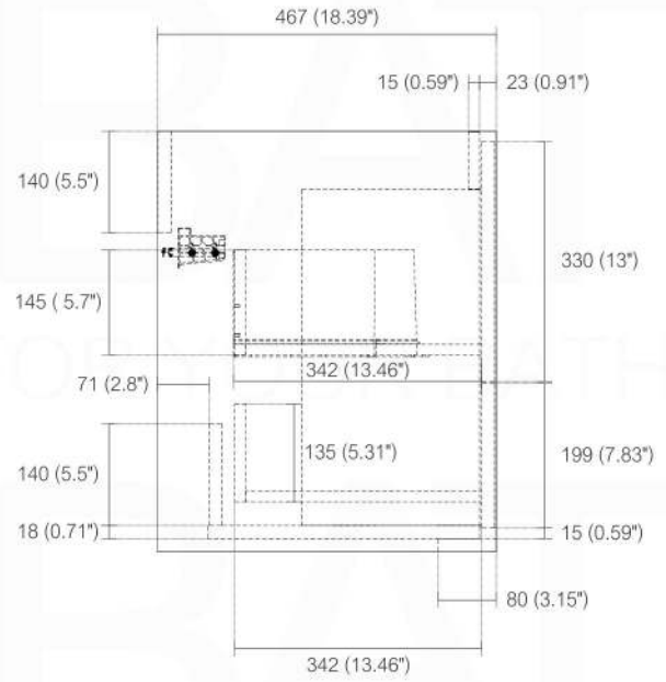
SIDE ELEVATION
