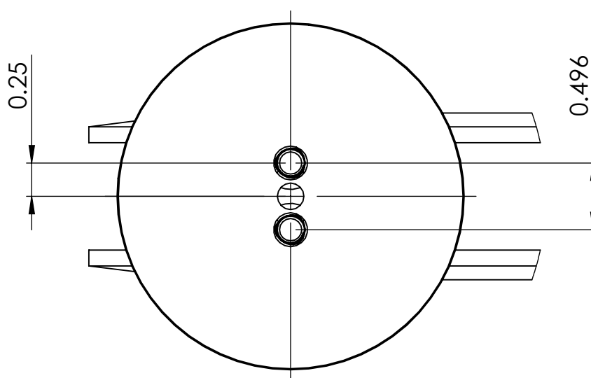
DETAIL O
