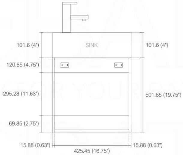
BACK ELEVATION
