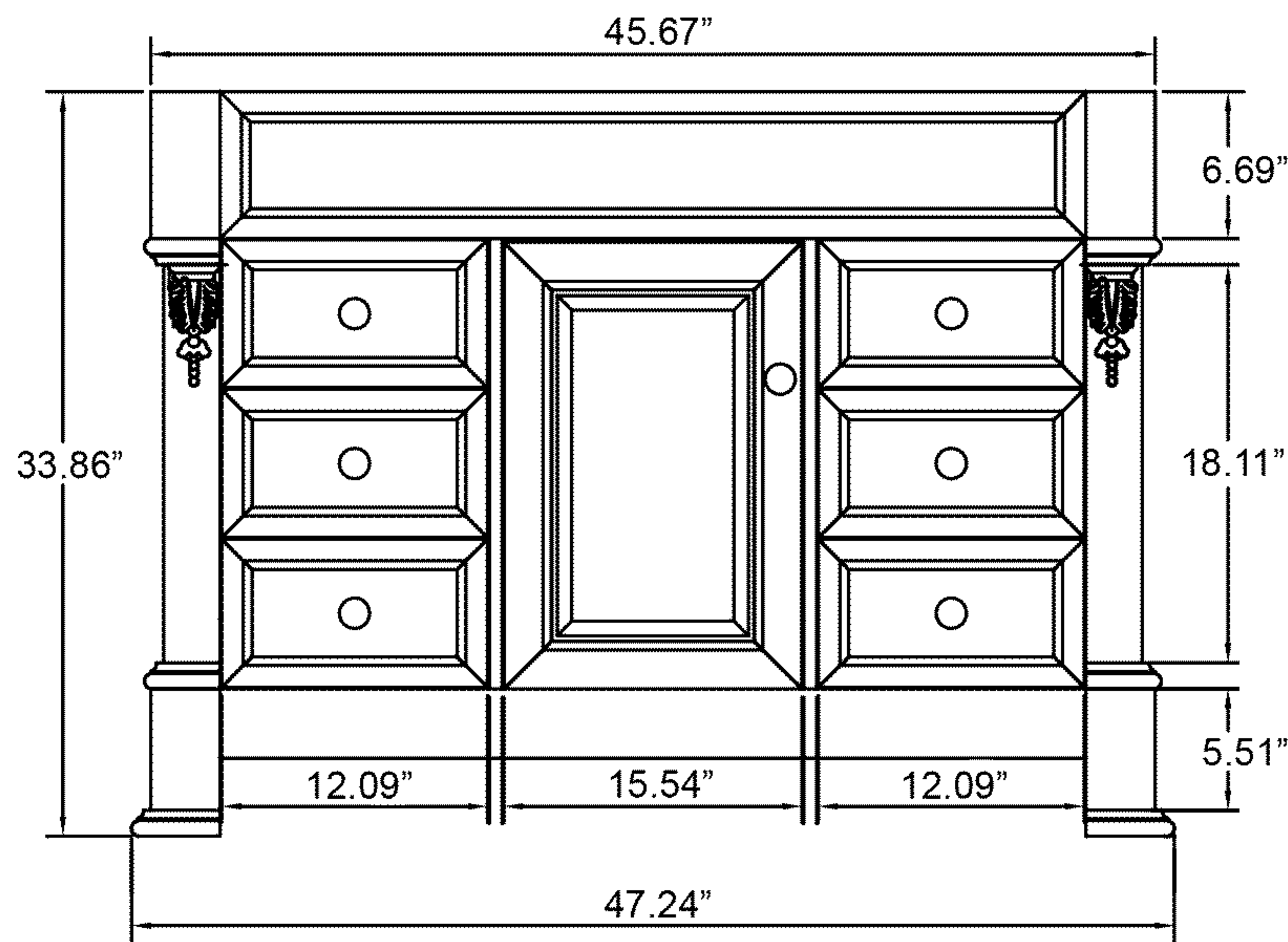
Front View
