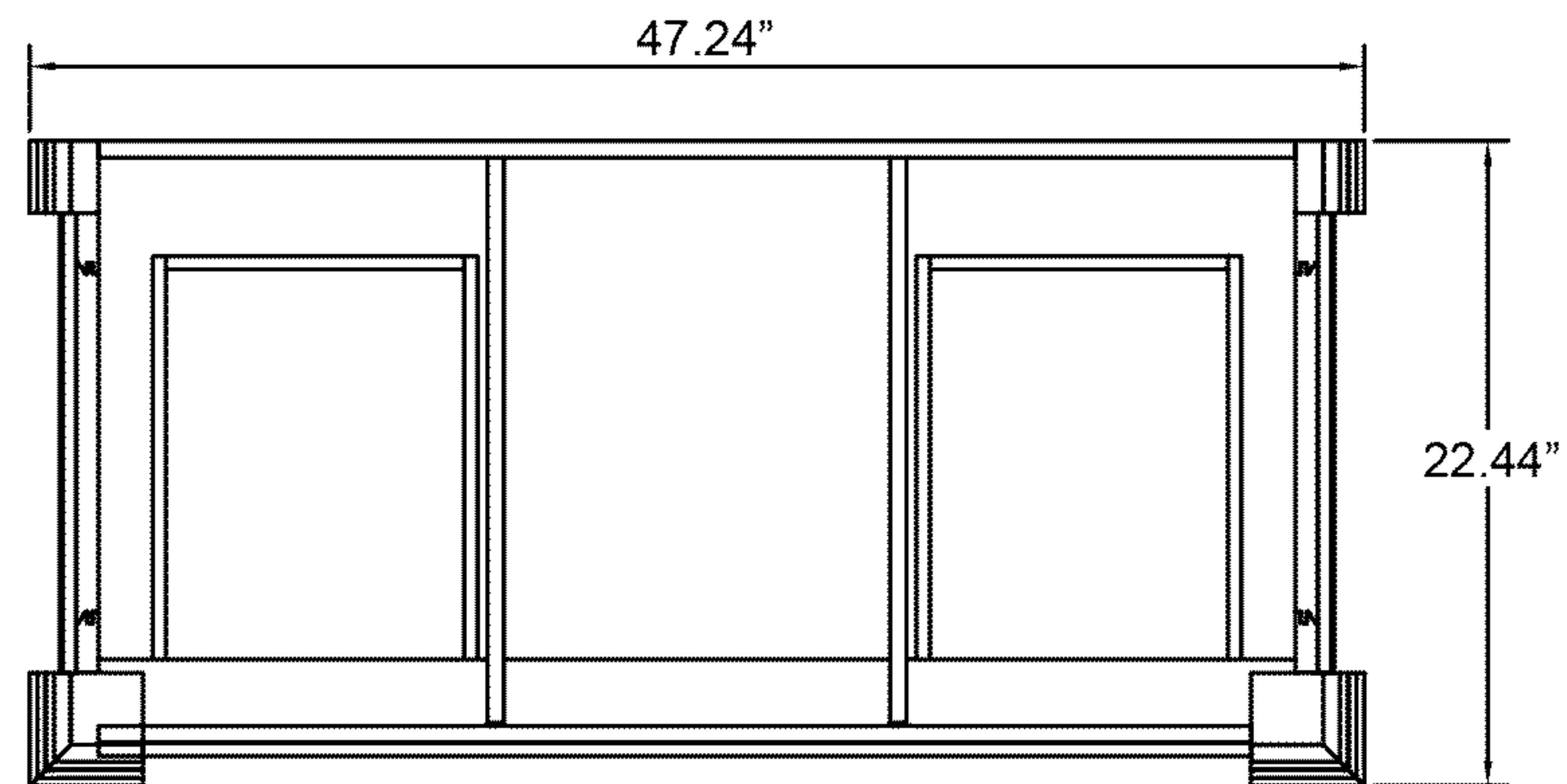
Back View
