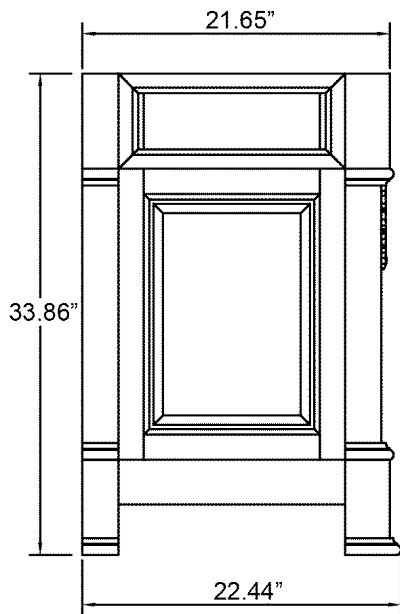
Side View
