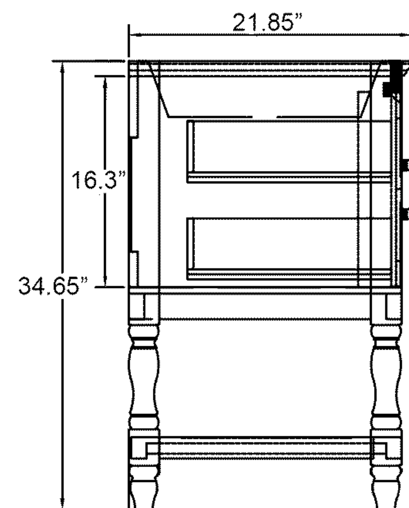
Side View
