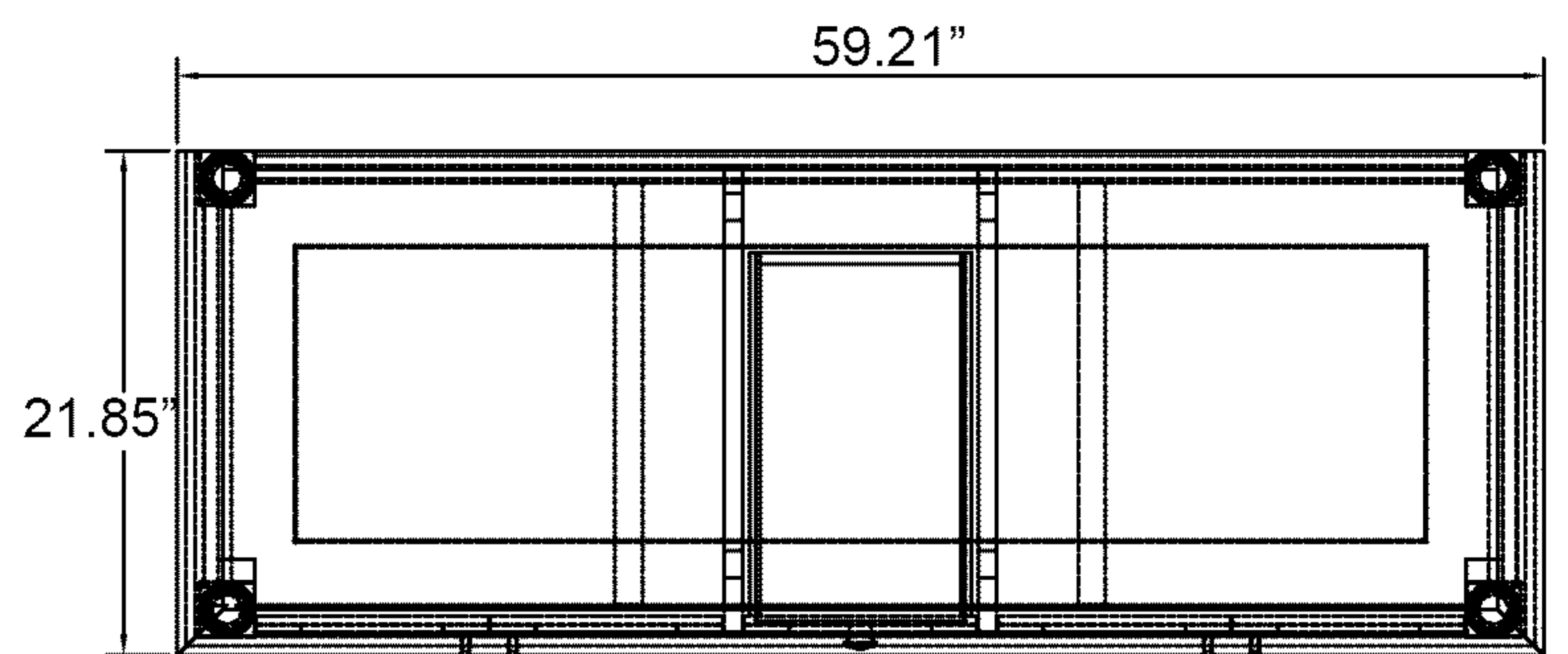
Top View
