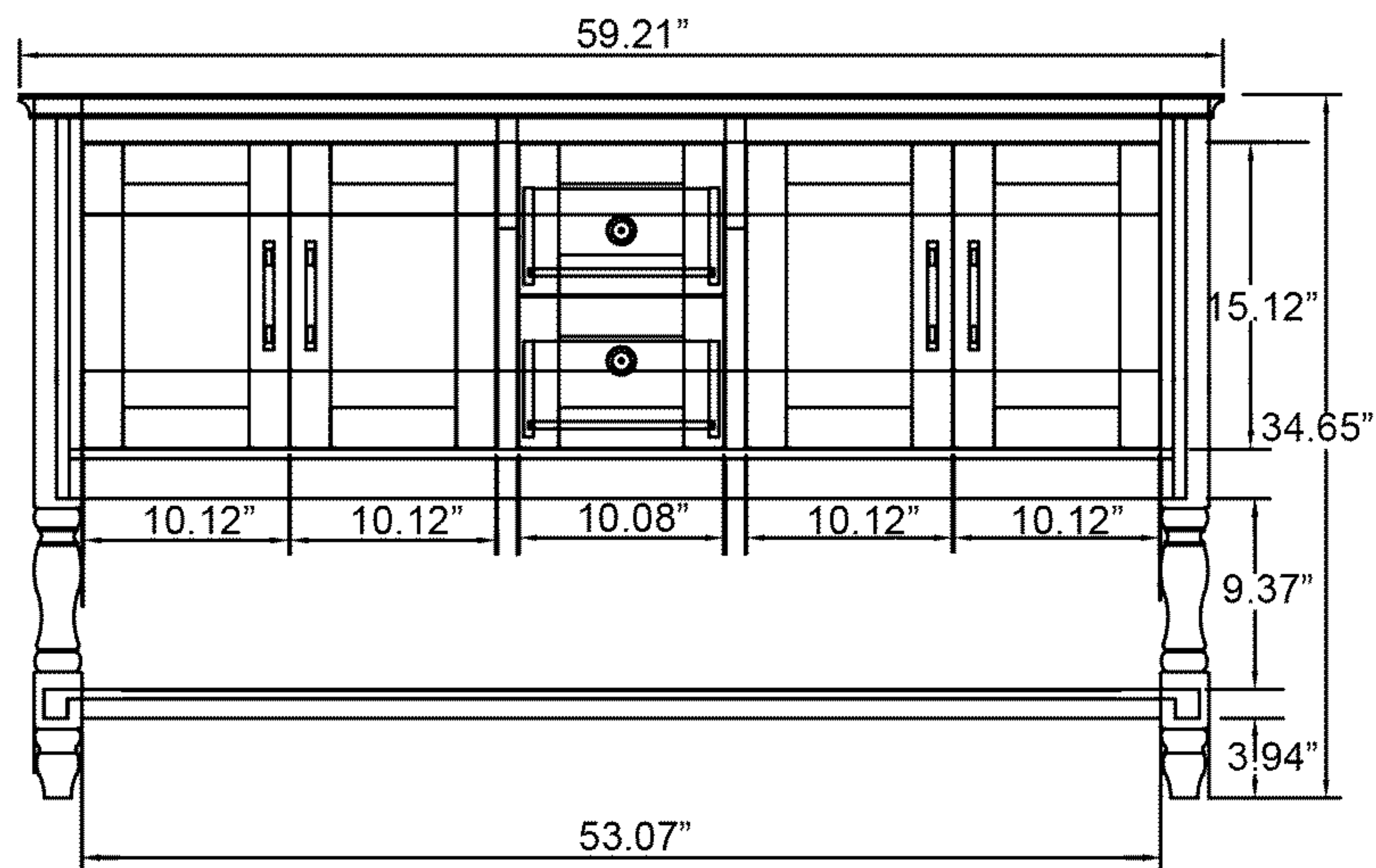
Front View
