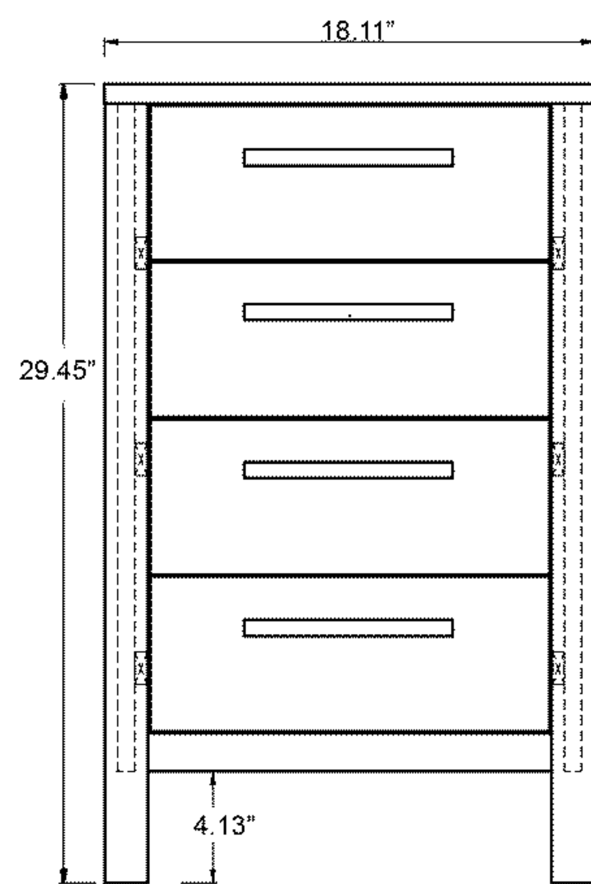
Front View
