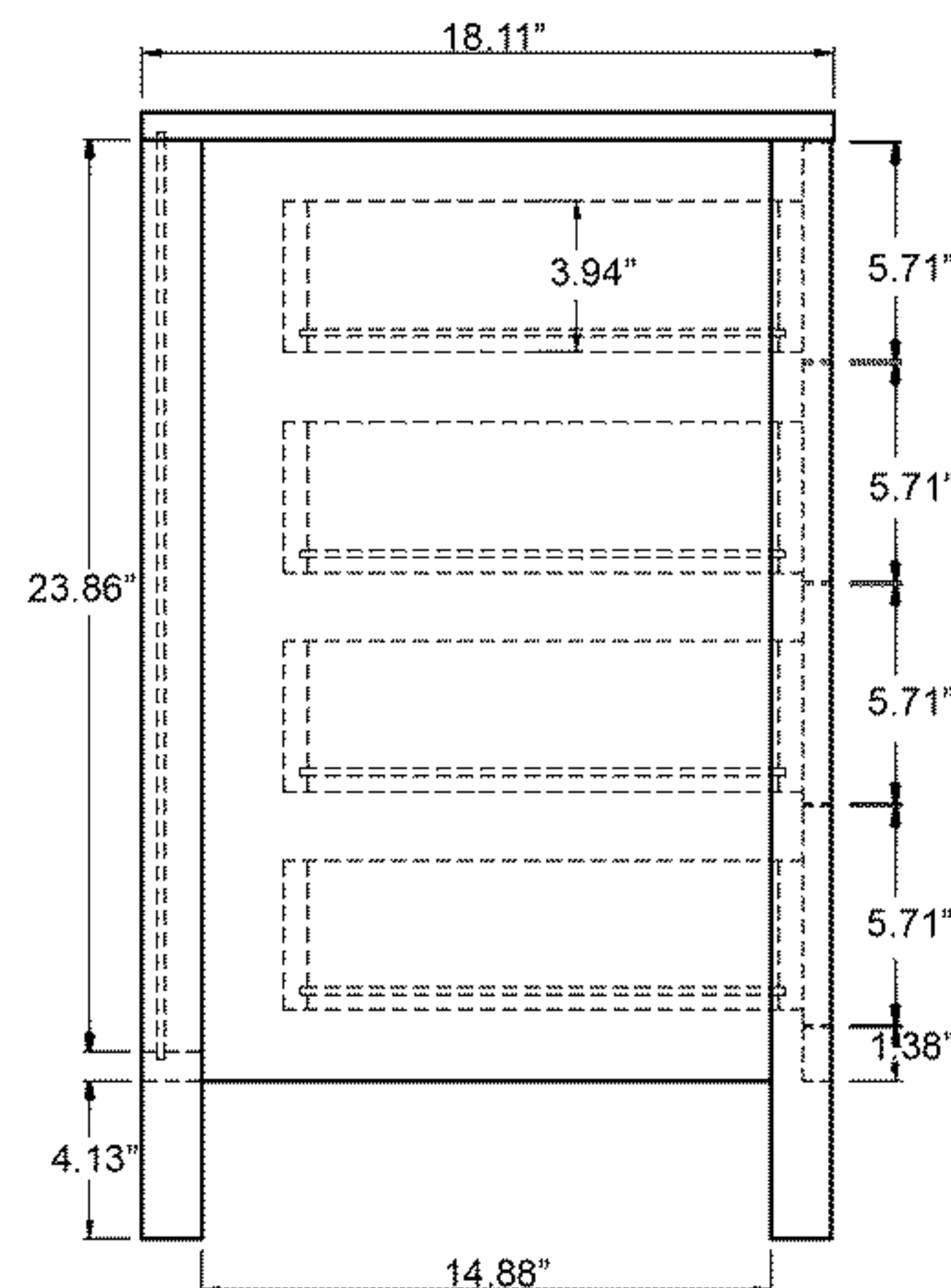
Side View
