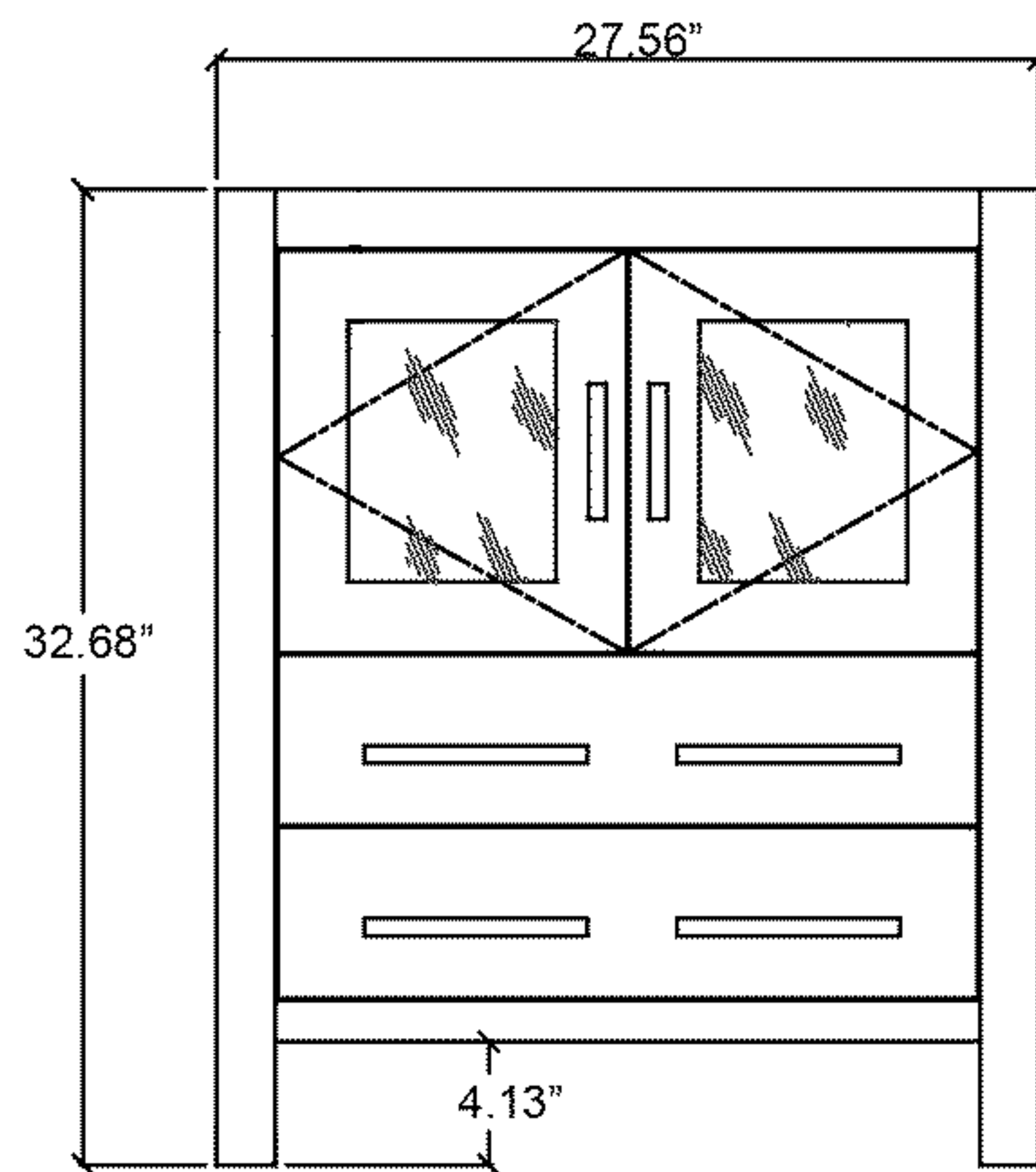
Front View
