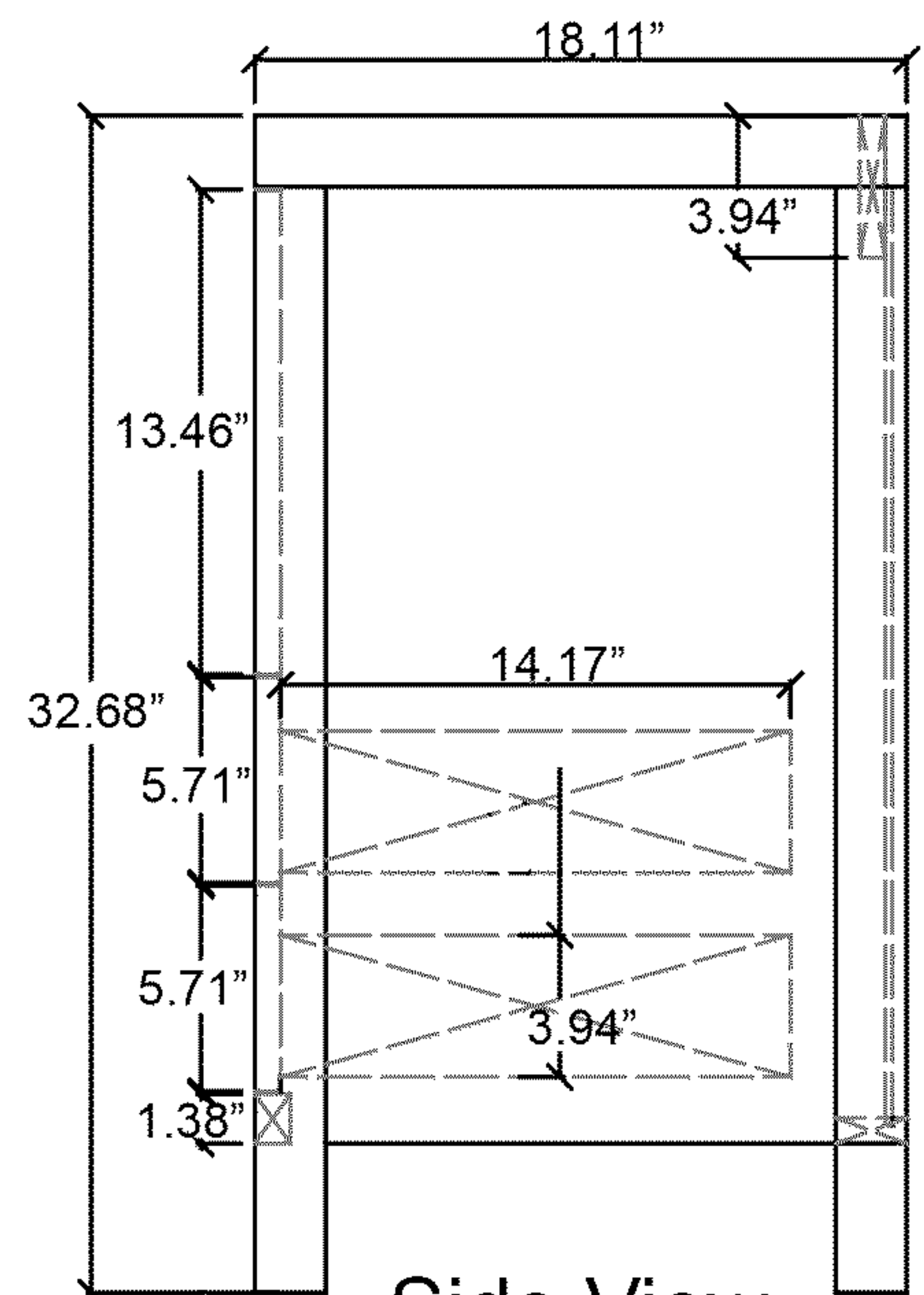
Side View
