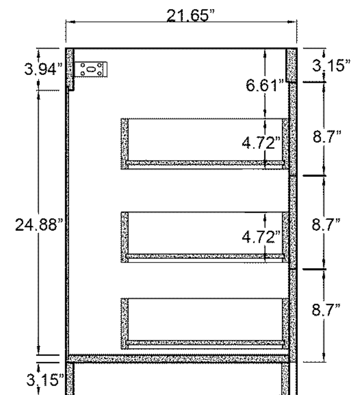
Side View
