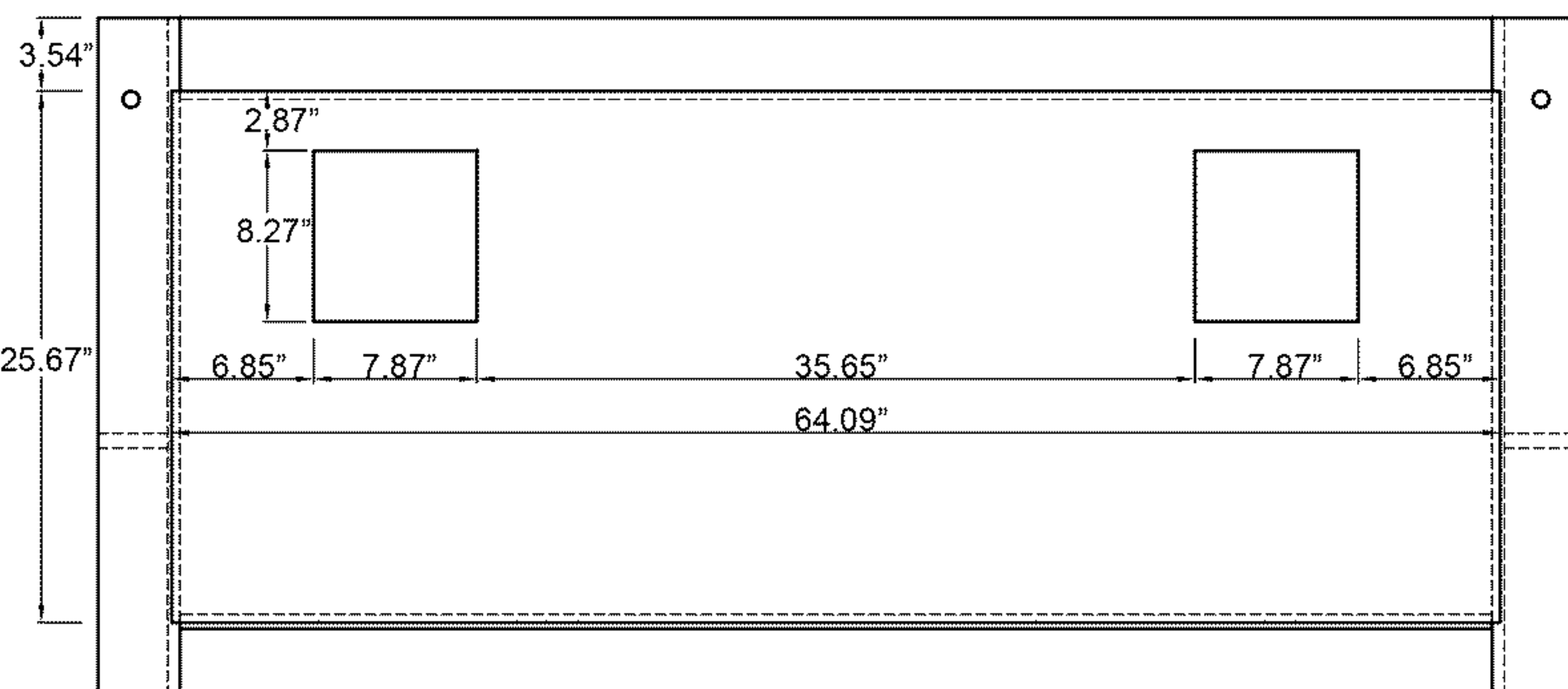
Back View
