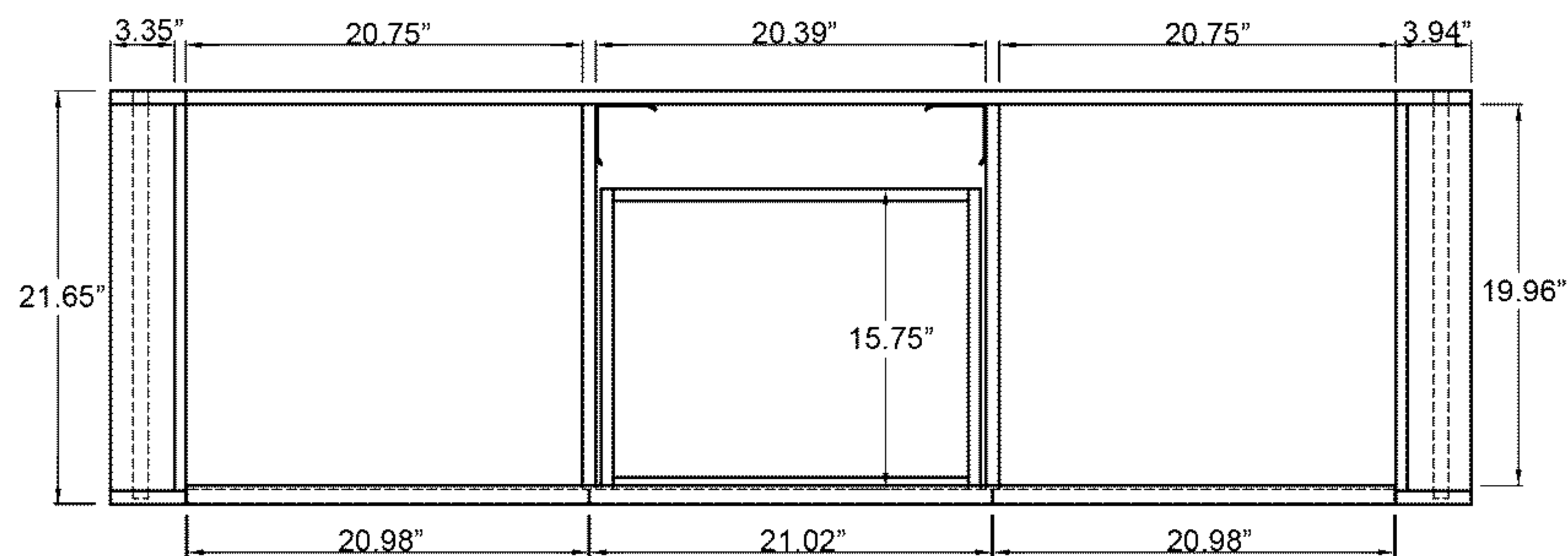
Top View
