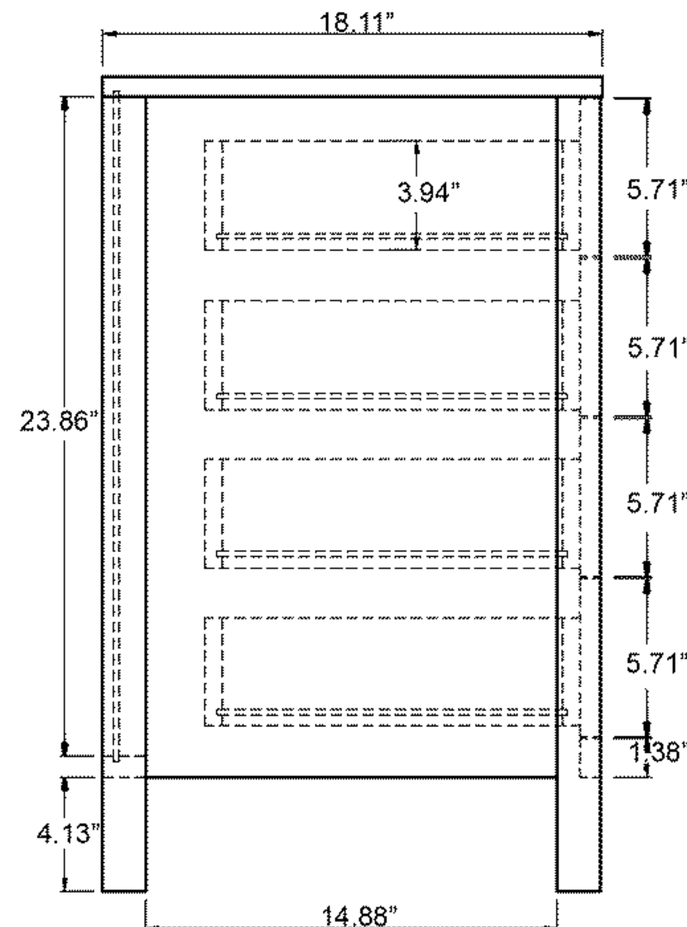
Side View
