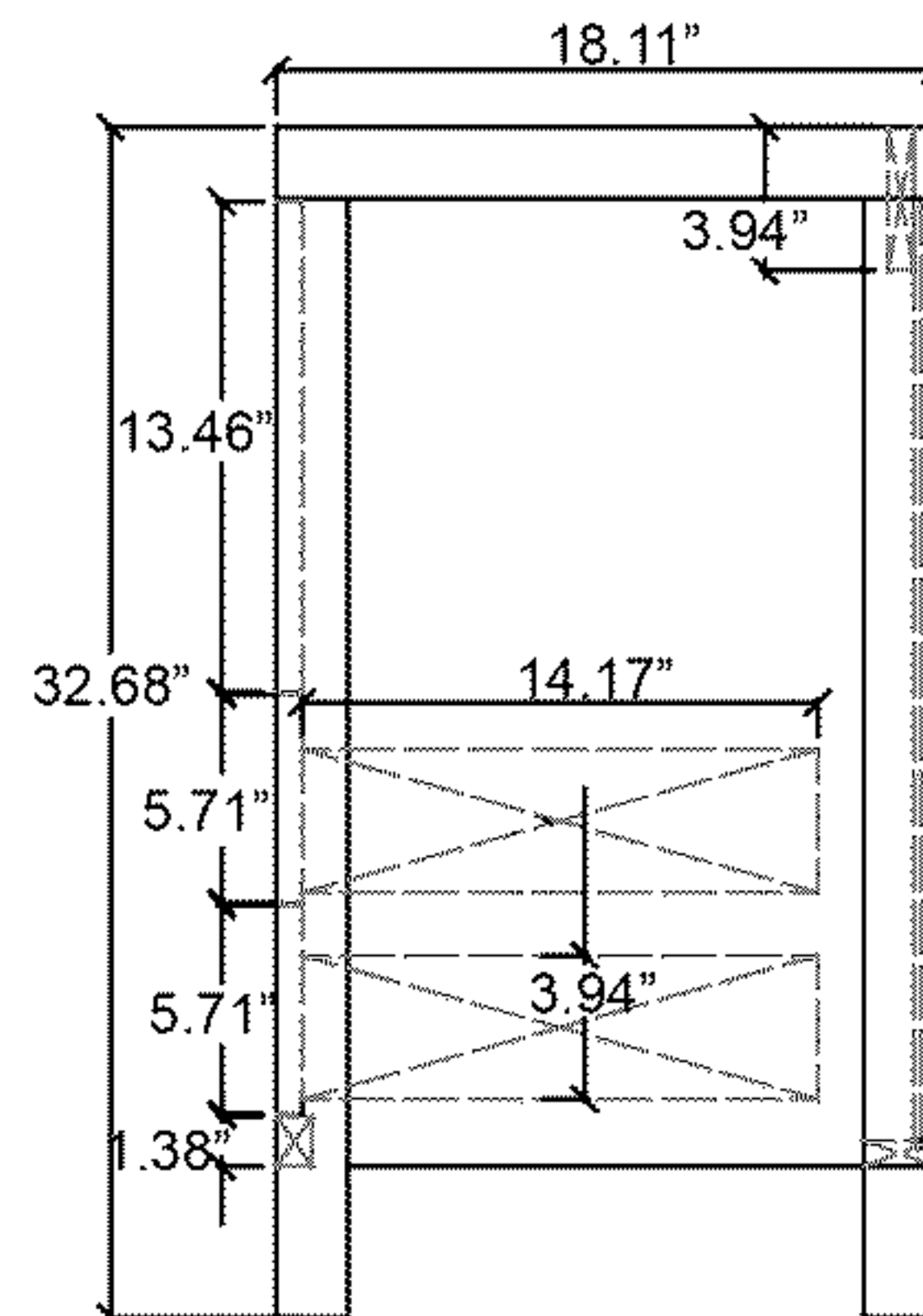
Side View
