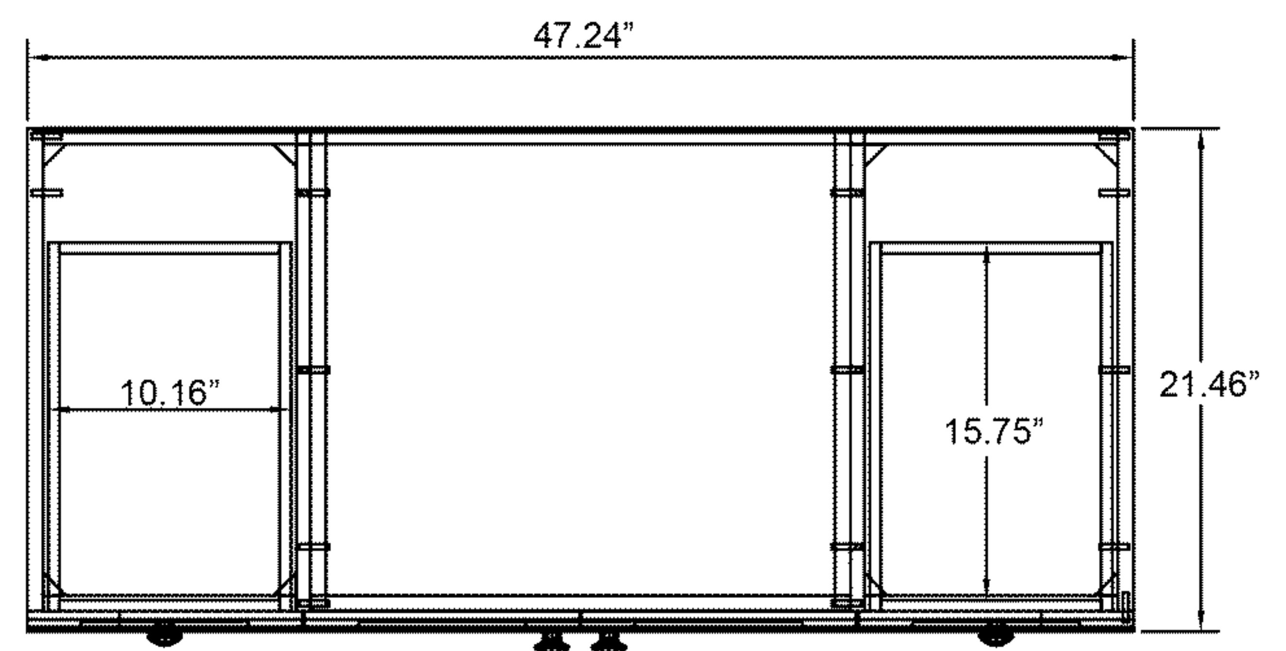
Top View
