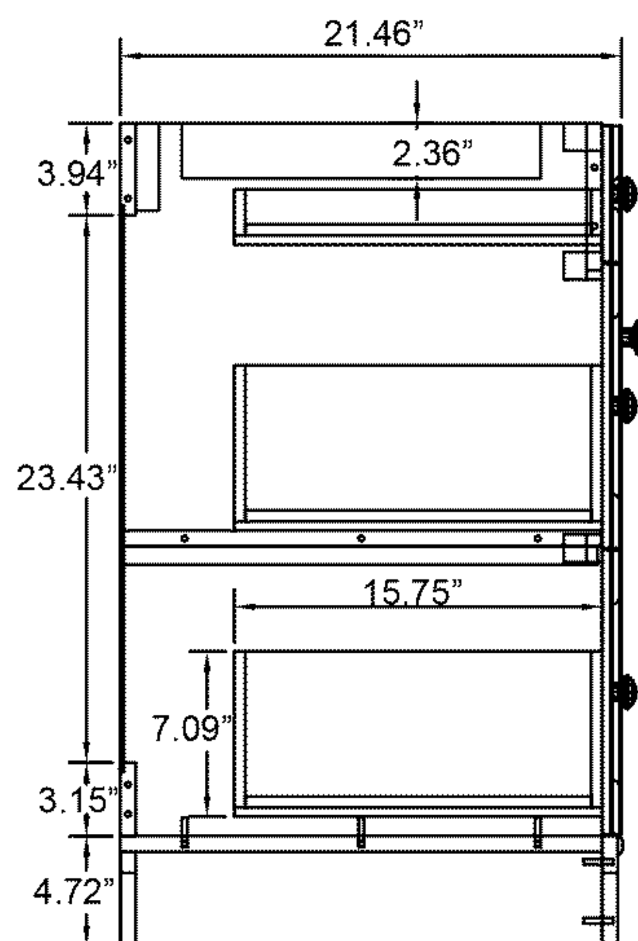
Side View
