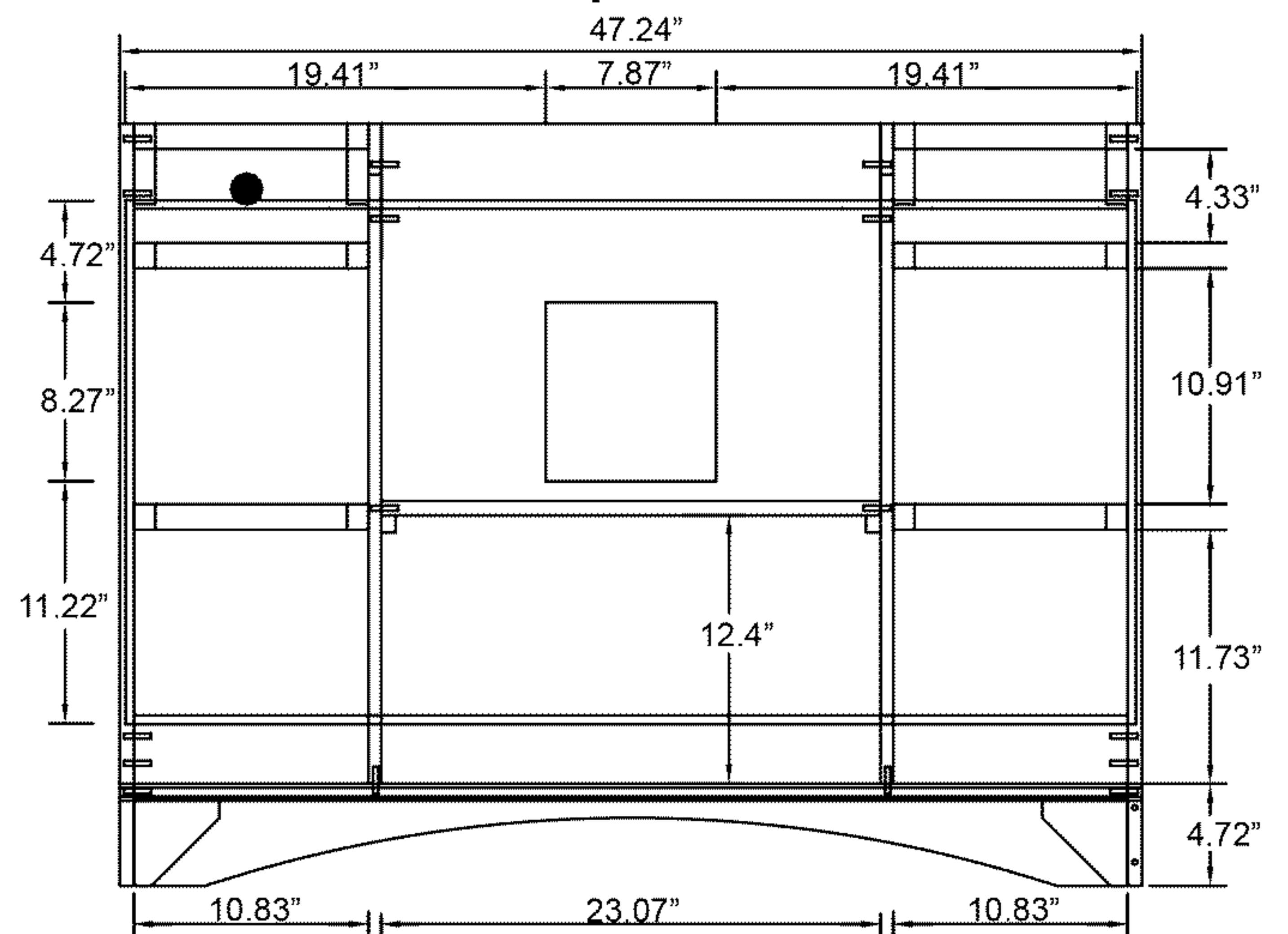
Back View
