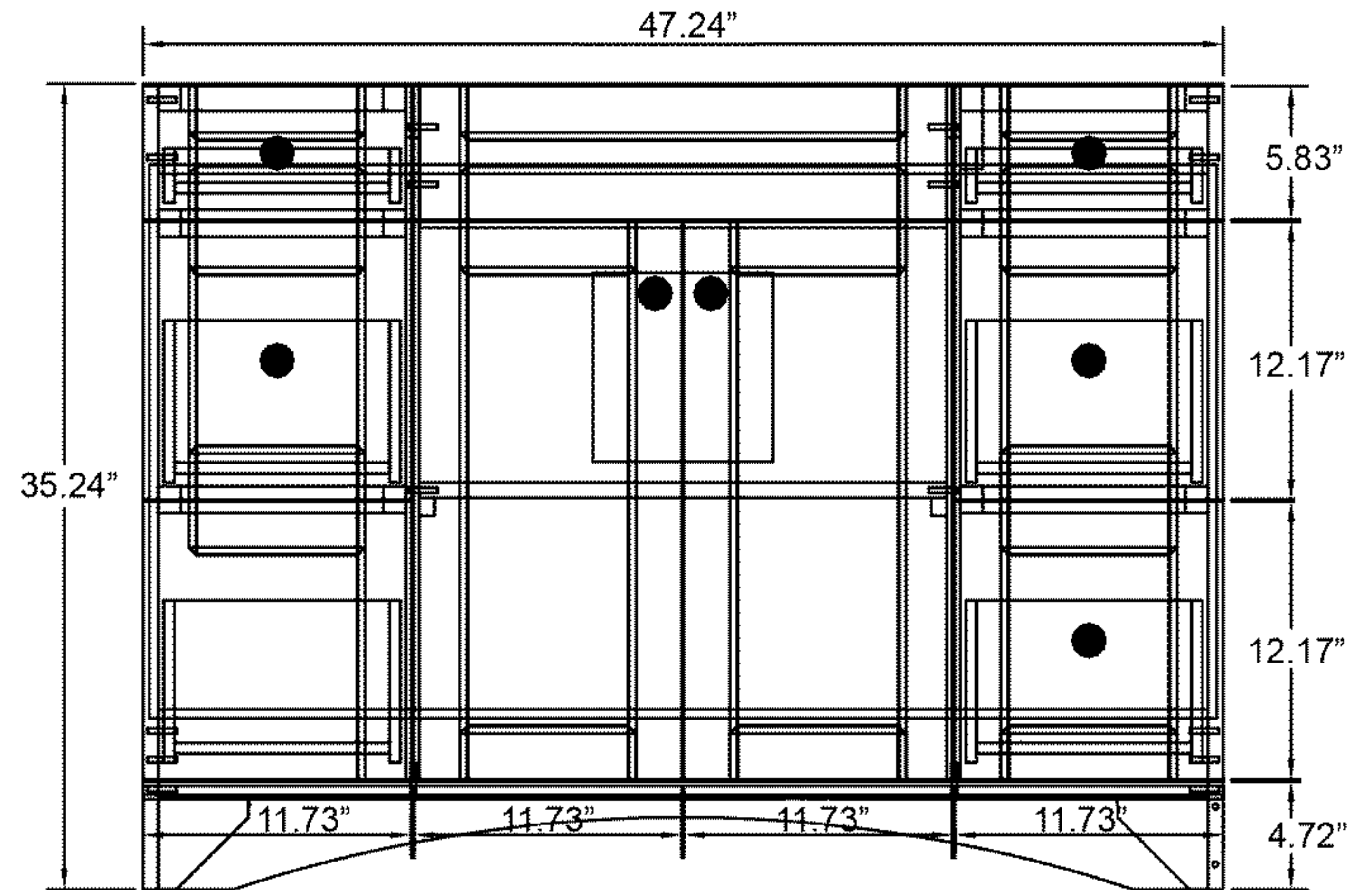
Front View
