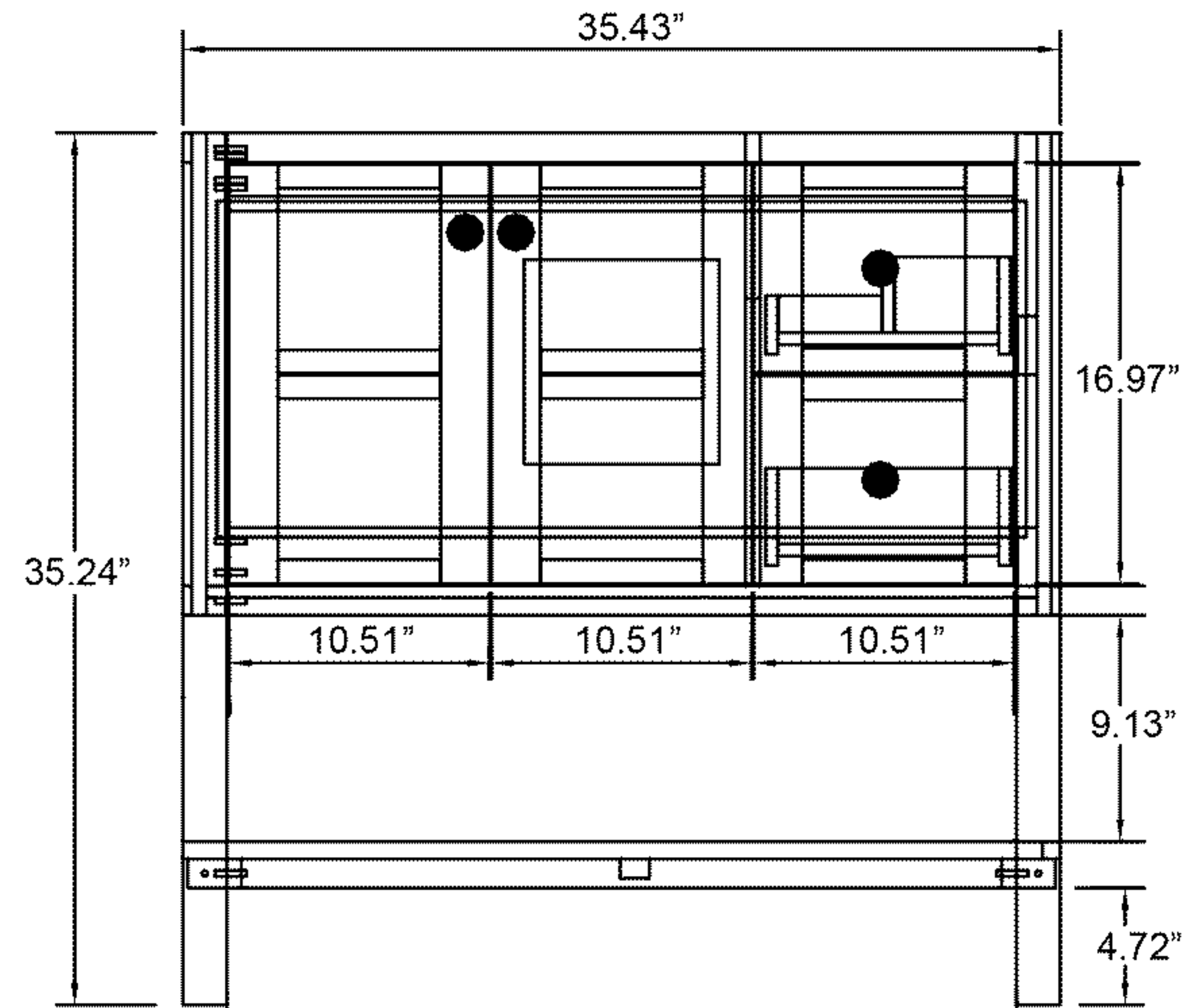
Front View
